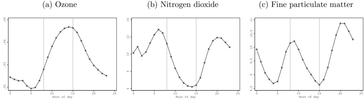
Figure A1: Hourly pollution concentrations
